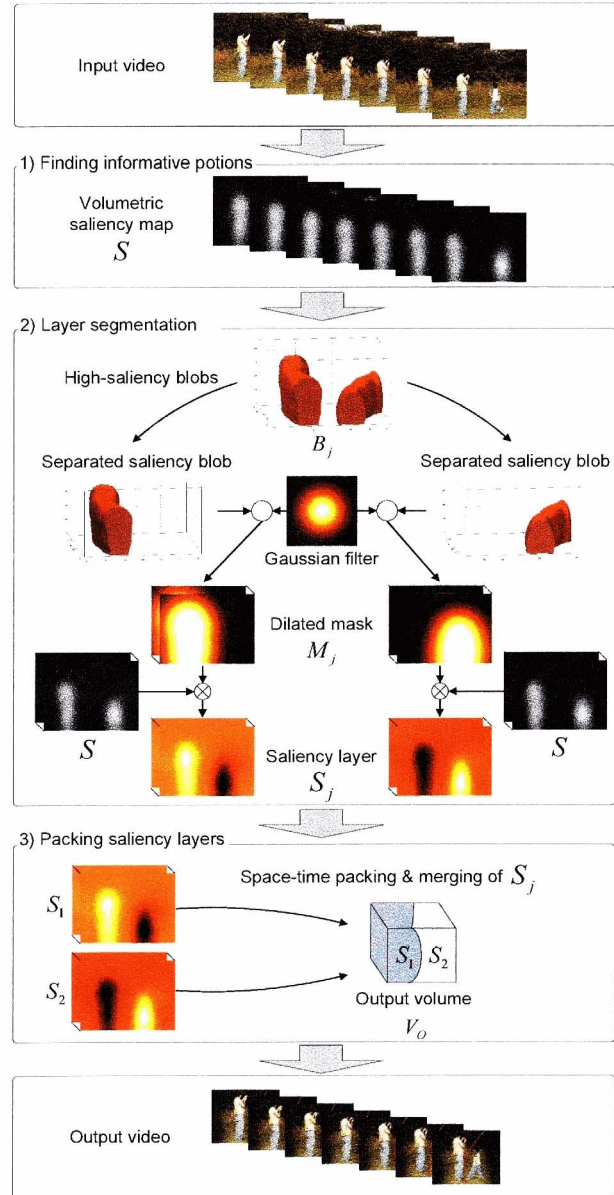
Figure 2. Overview of the space-time video montage.
