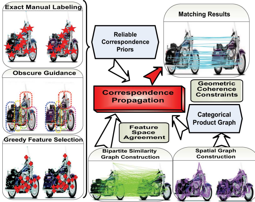
Fig. 2. Flowchart of correspondence propagation from reliable correspondence priors for feature matching.
