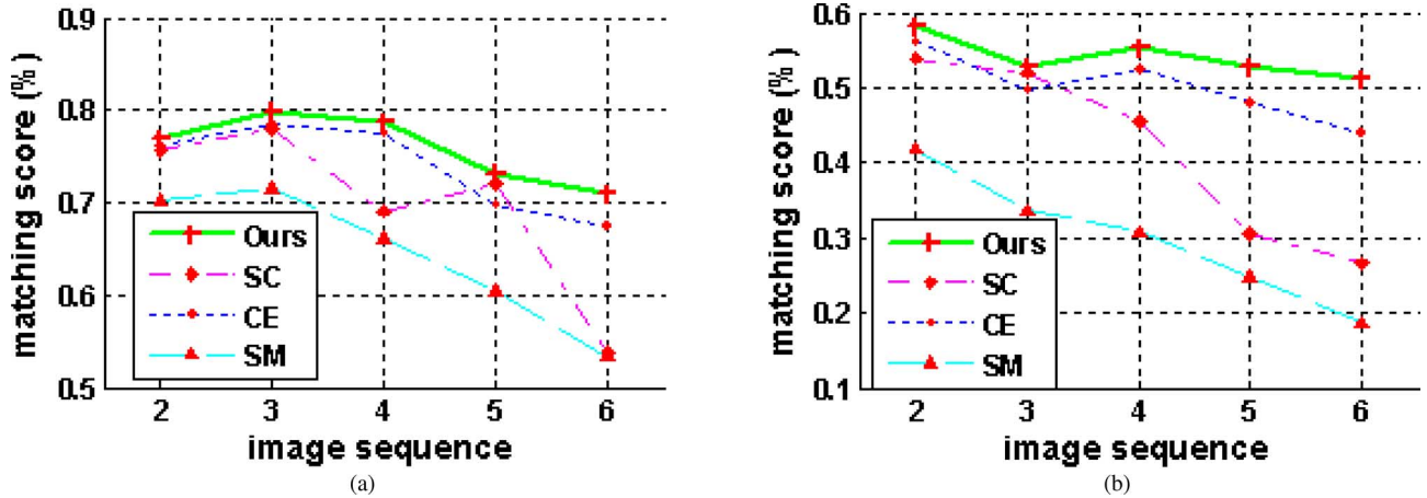
Fig. 7. Automatic feature matching score on the (a) bikes and (b) trees sequence for image blur. The blur sequence is acquired by varying the camera focus and the sequence is ordered with an increasing image blur.
