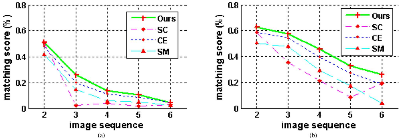
Fig. 9. Automatic feature matching score on the (a) bark and (b) boat sequence for zoom and rotation. The scale change (zoom) is acquired by varying the camera zoom and the zoom changes by about a factor of four. The image sequences are ordered with an increasing zoom and rotation.
