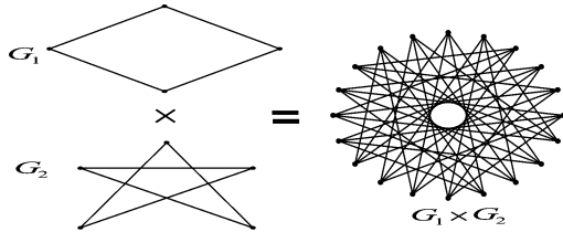
Fig. 3. Demonstration of categorical graph product: graph G_1 , graph G_2 , and their categorical graph product G_1 \times G_2 .
