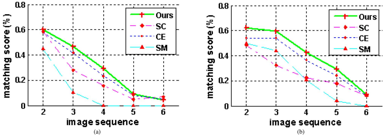
Fig. 6. Automatic feature matching score on the (a) Graffiti and (b) Wall sequence for viewpoint change. The camera varies from a fronto-parallel view to one with significant foreshortening at approximately 60 degrees to the camera. The image sequence is ordered with an increasing viewpoint variation.
